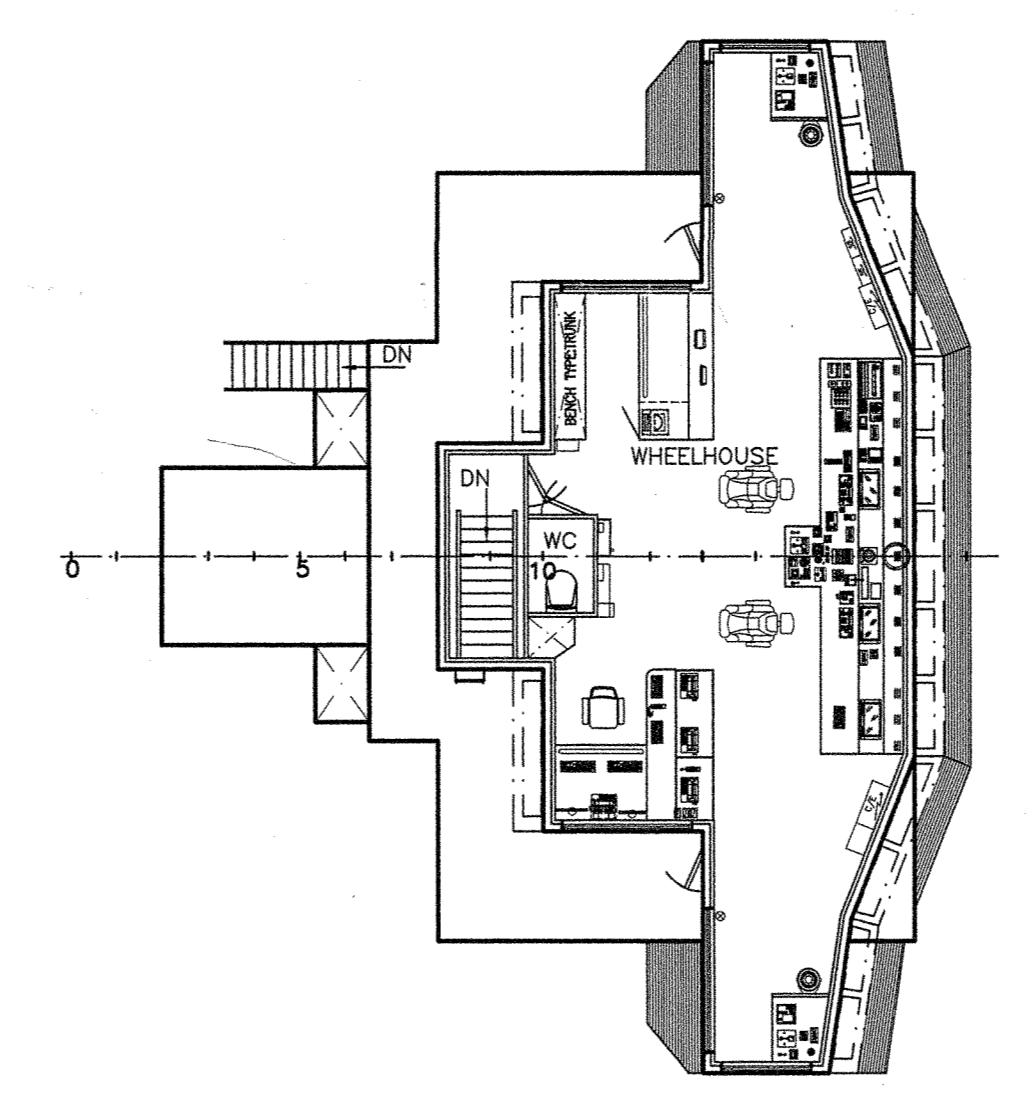
BRIDGE DECK
