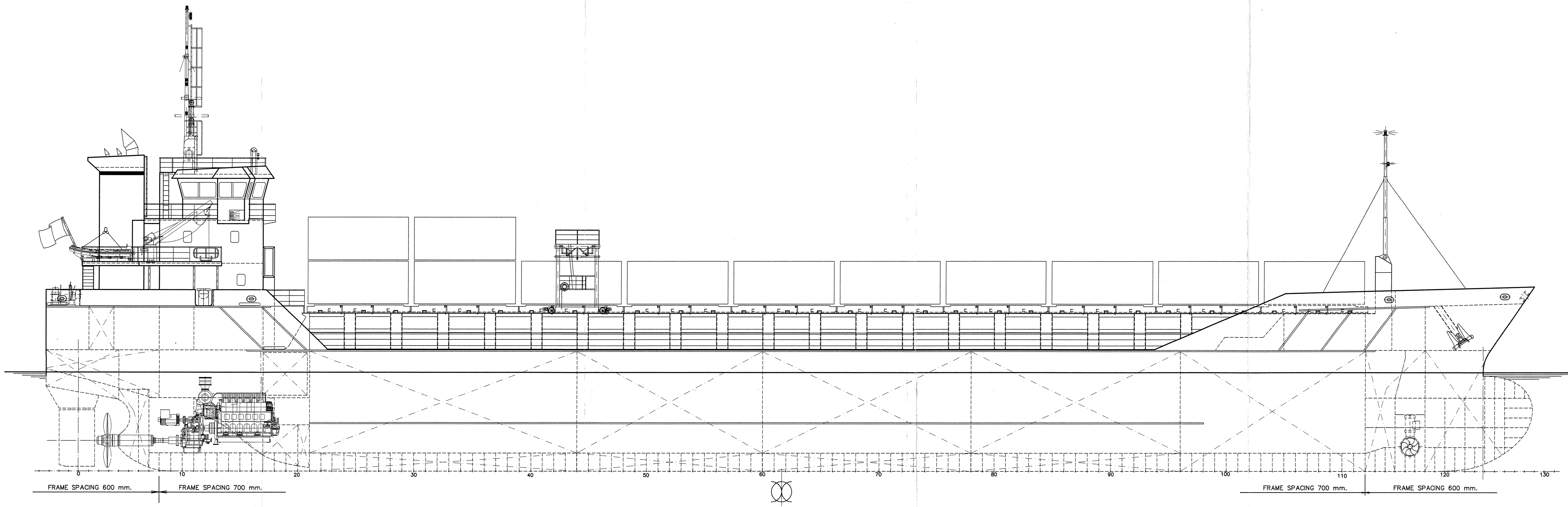
PROFILE
