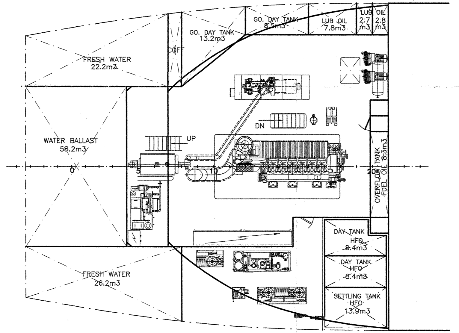
UPPER DECK
