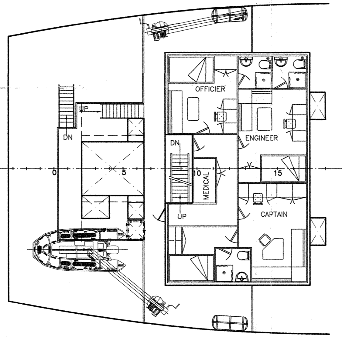
BOAT DECK
