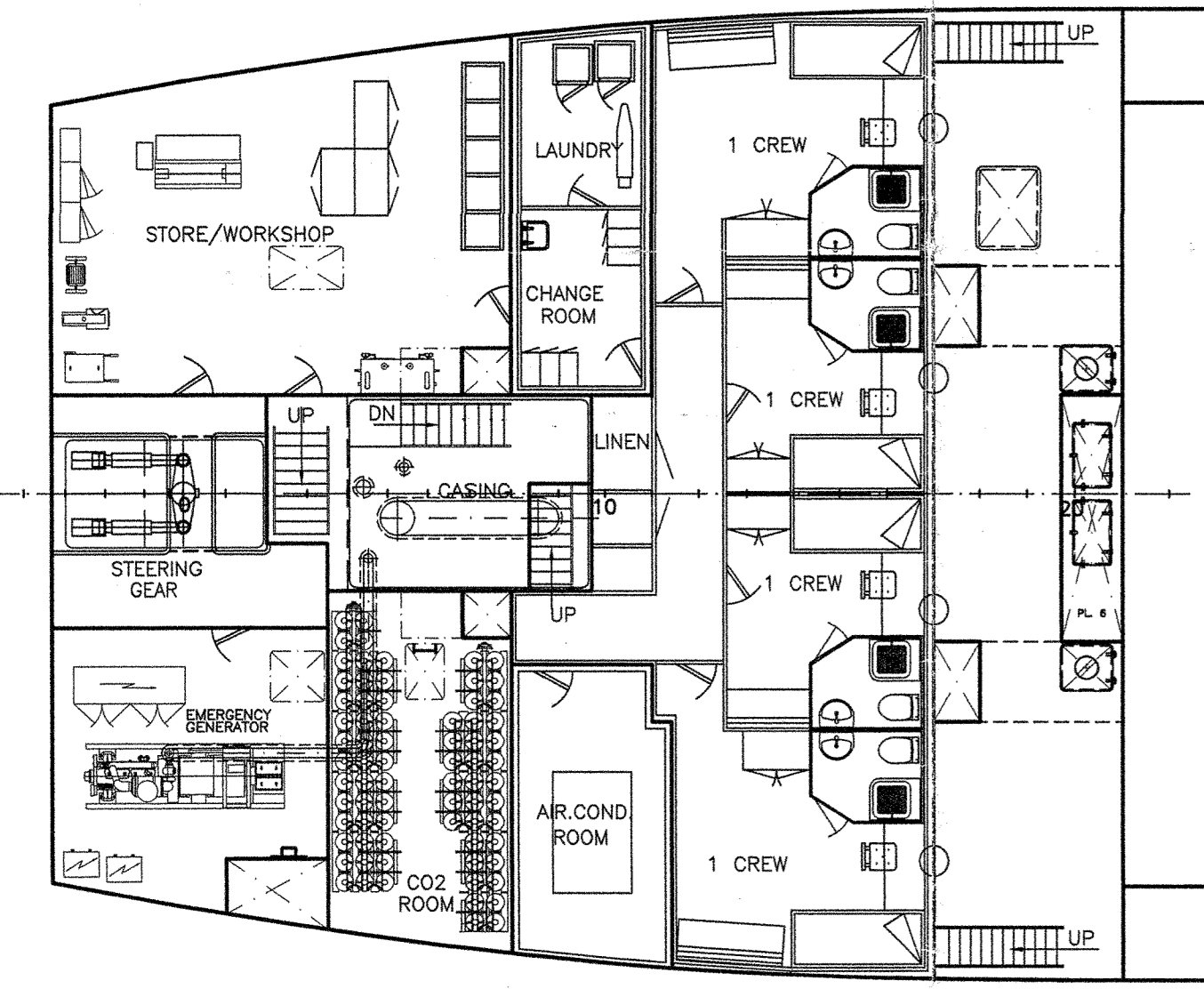
MAIN DECK
