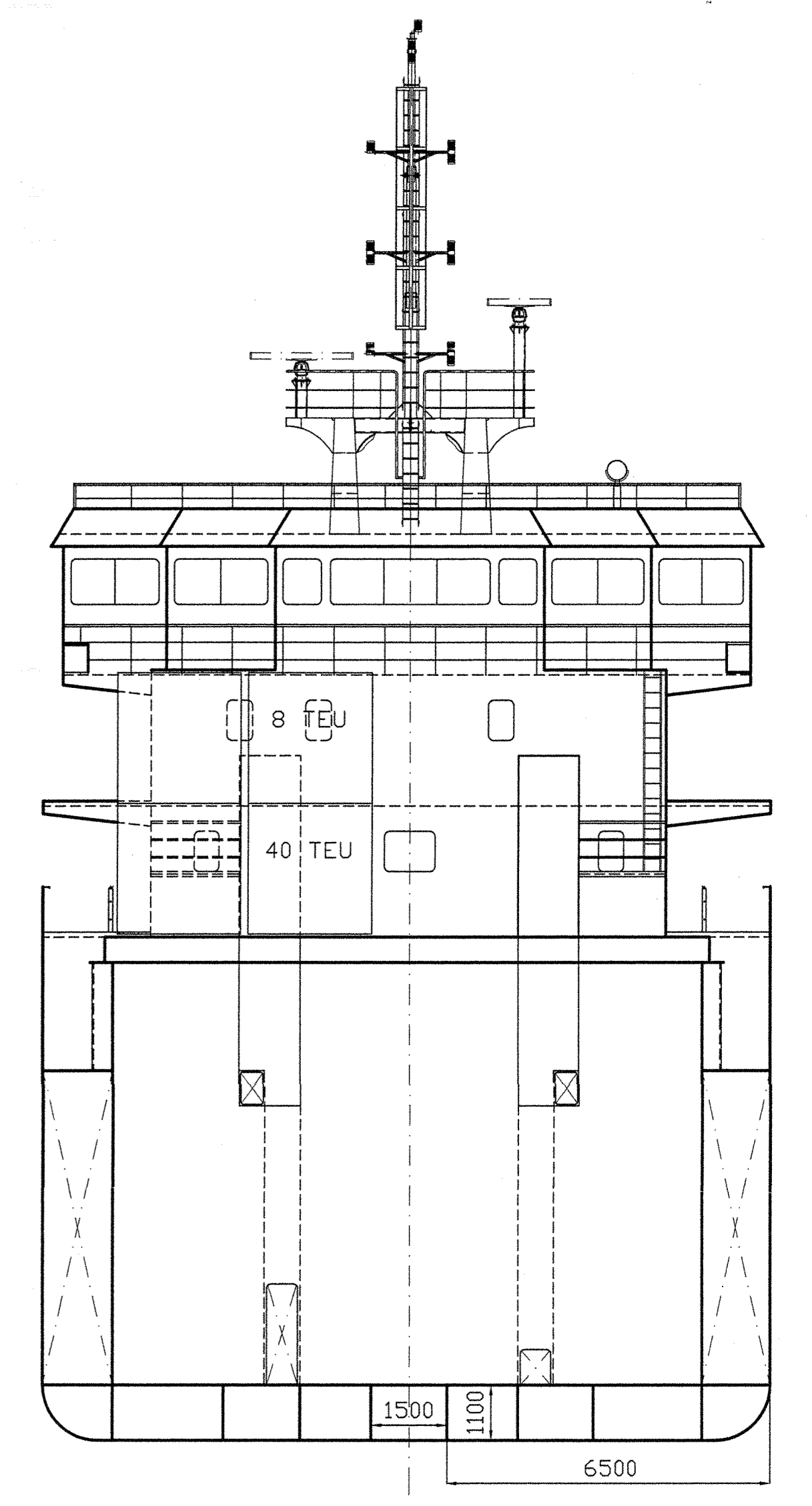
CROSS SECTION
