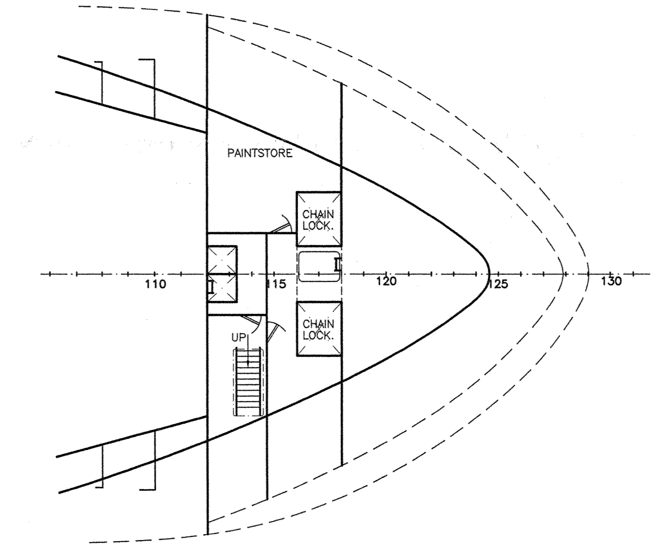
MAIN DECK
